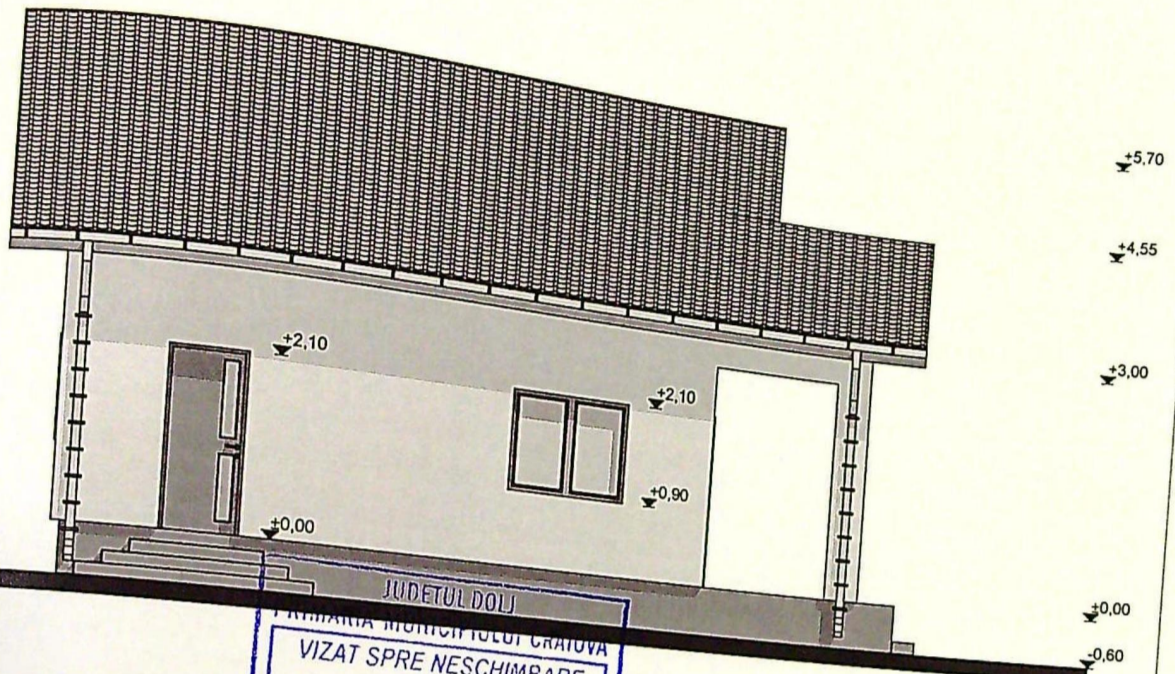
FATADA VEST
